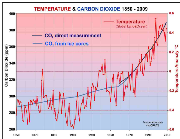
Many factors affect climate, but there is a strong relationship with CO 2 levels.
